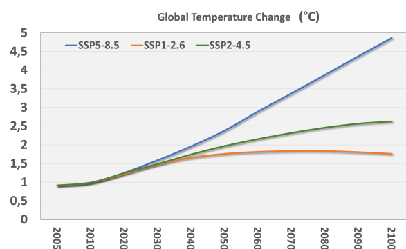
Global temperature increase compared to pre-industrial times. Schematic illustration.
